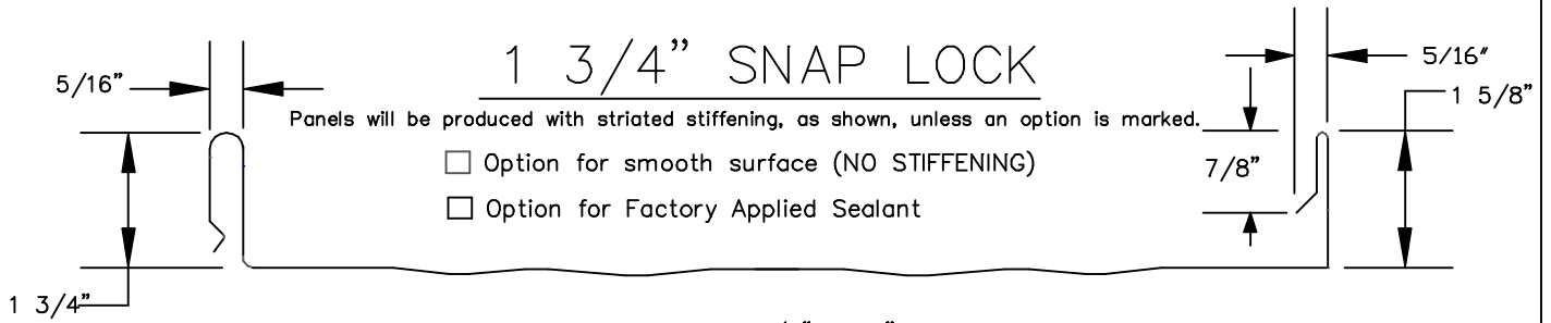
MODEL SL17518 1-3/4" X 18" SNAP LOCK
